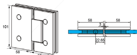
LSH S9803 (GG) 180° SATIN BRASS Available : • Brush Gun Metal • Chrome Polish
