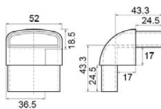
MOUNTING BRACKET SD S001-02A (2 pcs)
