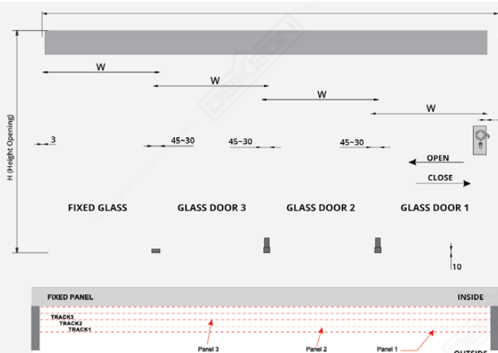
DOOR PANEL TRACK SGT 4100 (3+1) NA (2 pc)
