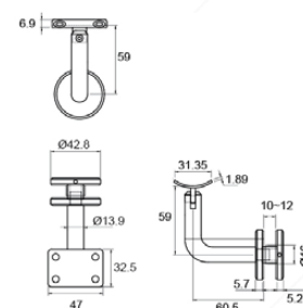
GLASS HOLDER BANISTER GH 14-01 OVAL SSS Available: GH 14-01 STRAIGHT SSS
