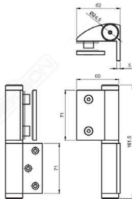
SHH 502 MATT BLACK (GLASS TO WALL)
