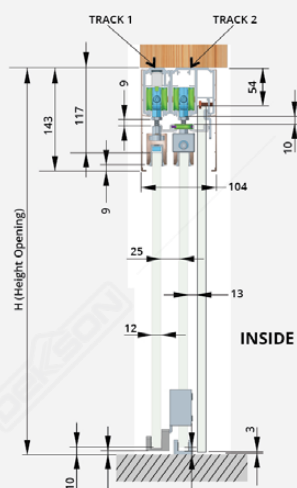
FIX PANEL TRACK SGT 3100 (2+1) NA (1 pc)
