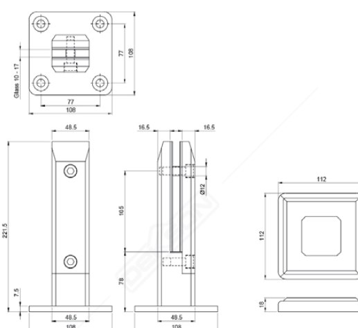
GC ST001 SSS Available: GC ST001 MATT BLACK
