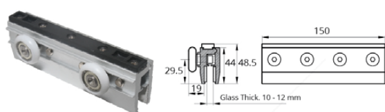
CLAMP ROLLER (2 pcs)
