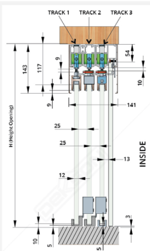
FIX PANEL TRACK SGT 4100 (3+1) NA (1 pc)
