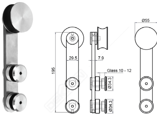
ROLLER FOR TUBE (2 pcs)
