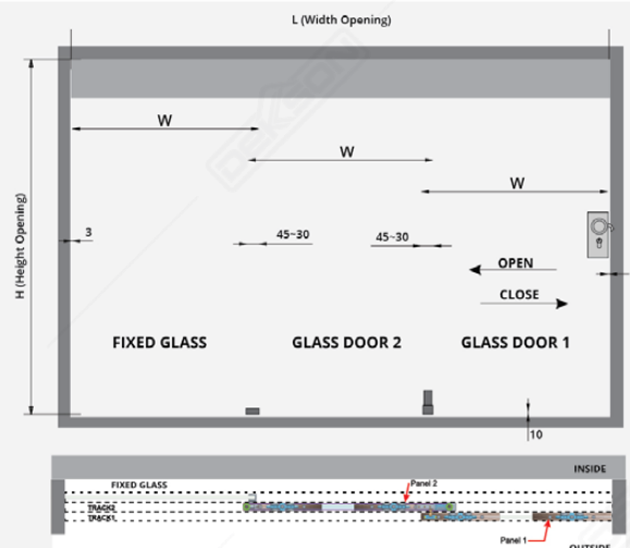
DOOR PANEL TRACK SGT 3100 (2+1) NA (1 pc)
