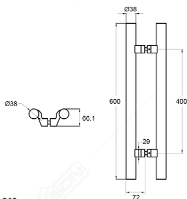
PH DL810 38x600x400 PSS+SSS Available in : 38x800x600 PSS+SSS 38x1000x800 PSS+SSS Material : SUS 304
